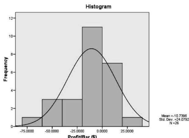
FIGURE 2: '4FAFM' excluding outliers
