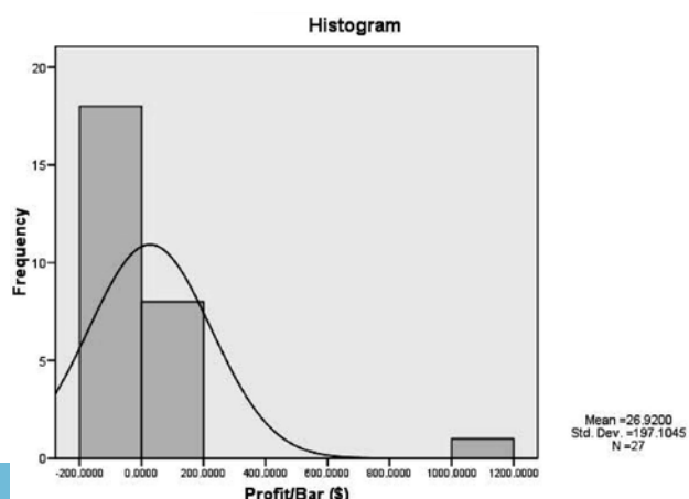
FIGURE 1: '4FAFM' model with outliers
